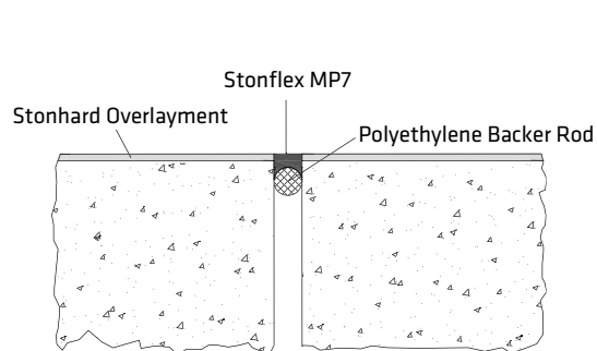
JOINT EXPANSION / ISOLATION JOINT DETAIL
